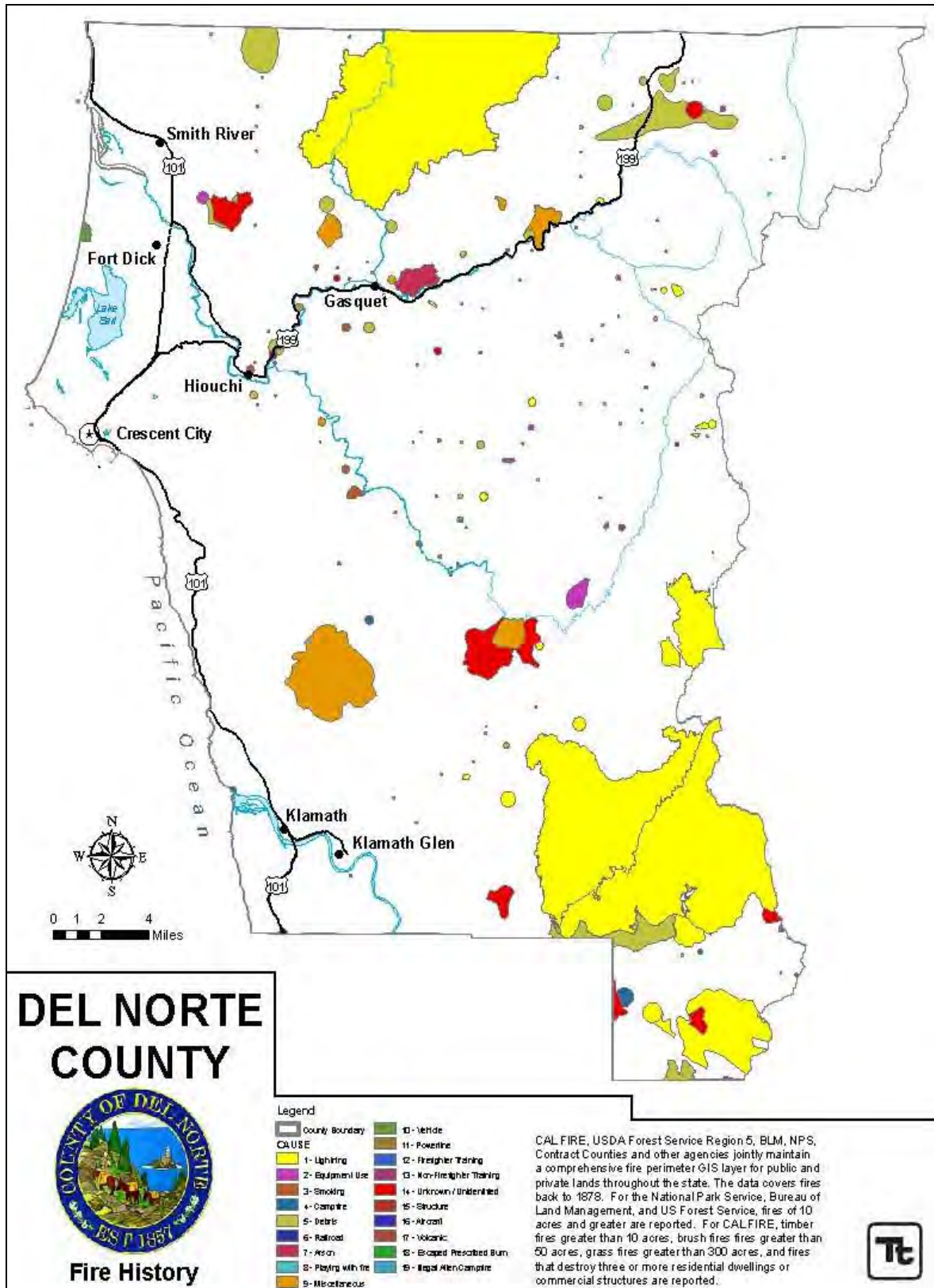
Figure 17-3. Extent and Location of Del Norte County Wildland Fires, 1901 – 2009
