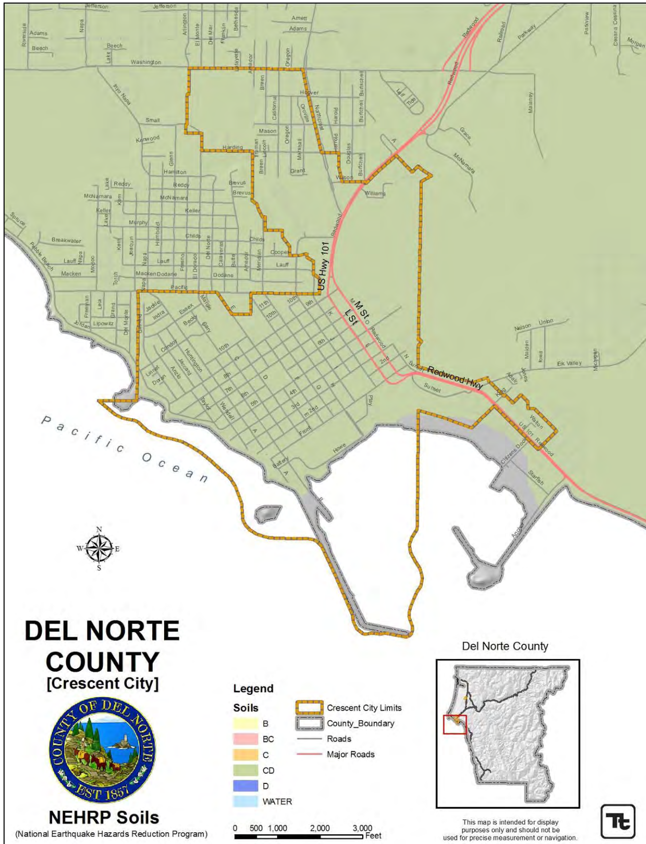
Figure 3-3. Crescent City NEHRP Soil Types
