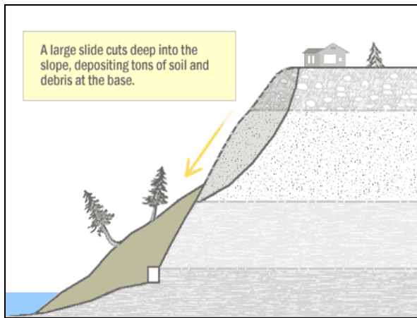
Figure 14-3. Translational Slides
