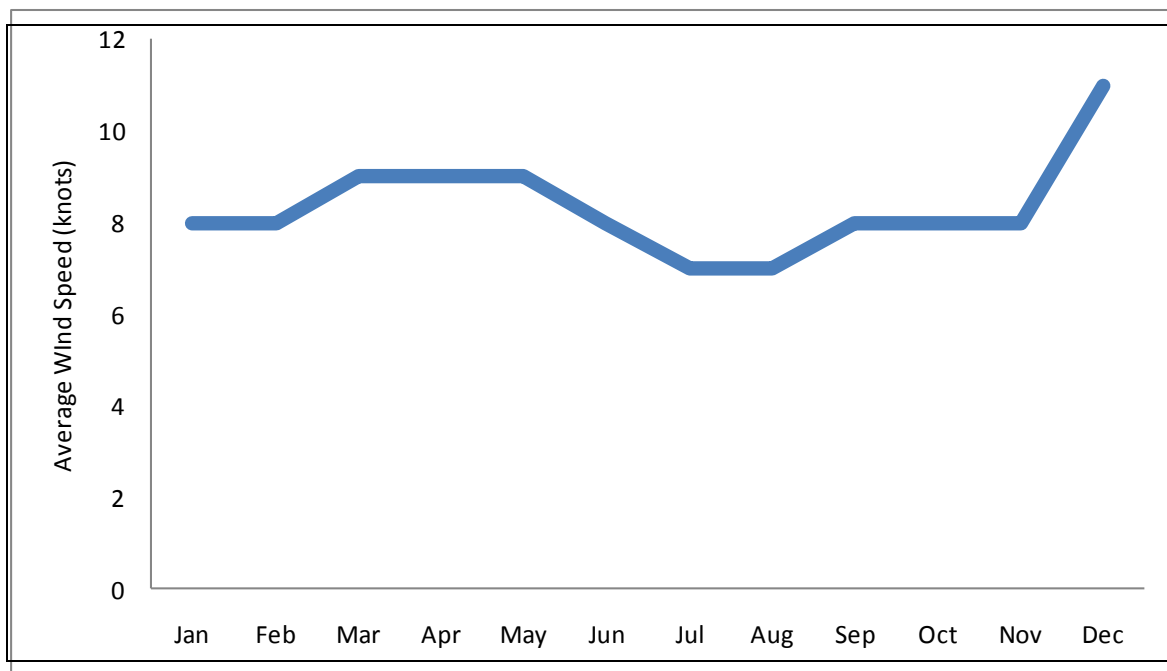
Figure 15-1. Average Wind Speed for Crescent City, January 2006 – August 2009 (NCDC 2007)
