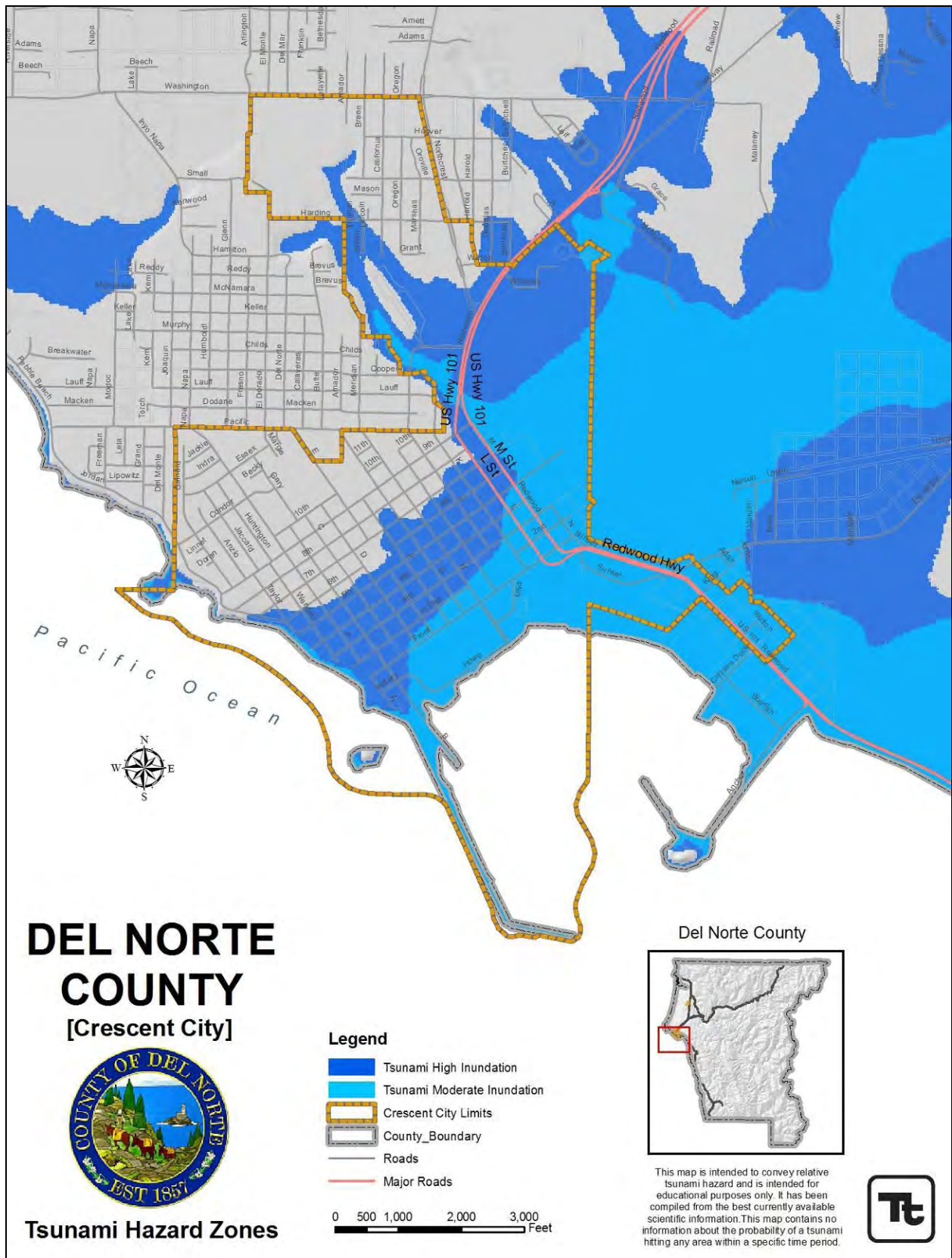
Figure 3-5. Crescent City Tsunami Hazard Areas
