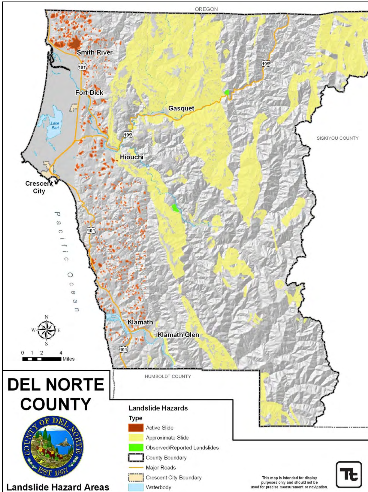
Figure 14-5. Slope Stability
