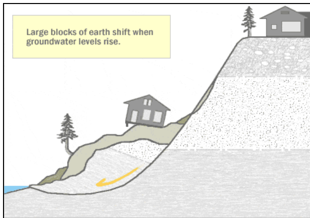
Figure 14-1. Large Rotational Slide (Deep Seated)
