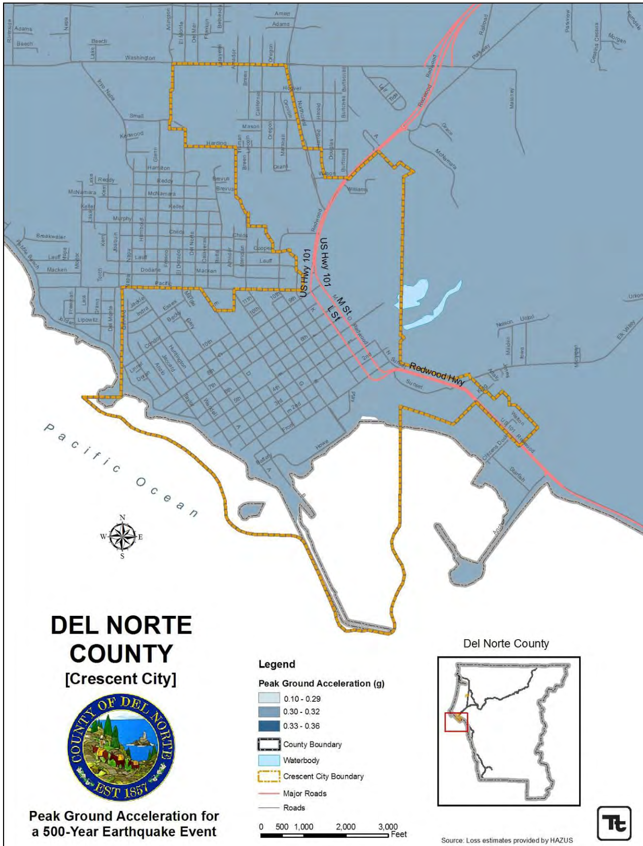
Figure 3-2. Crescent City Earthquake Hazard Areas-500-year probabilistic
