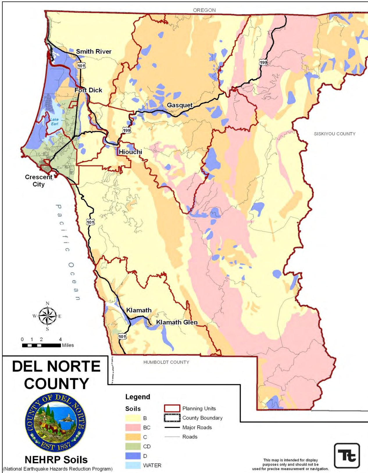
Figure 12-3. NEHRP Soil Classifications in Del Norte County
