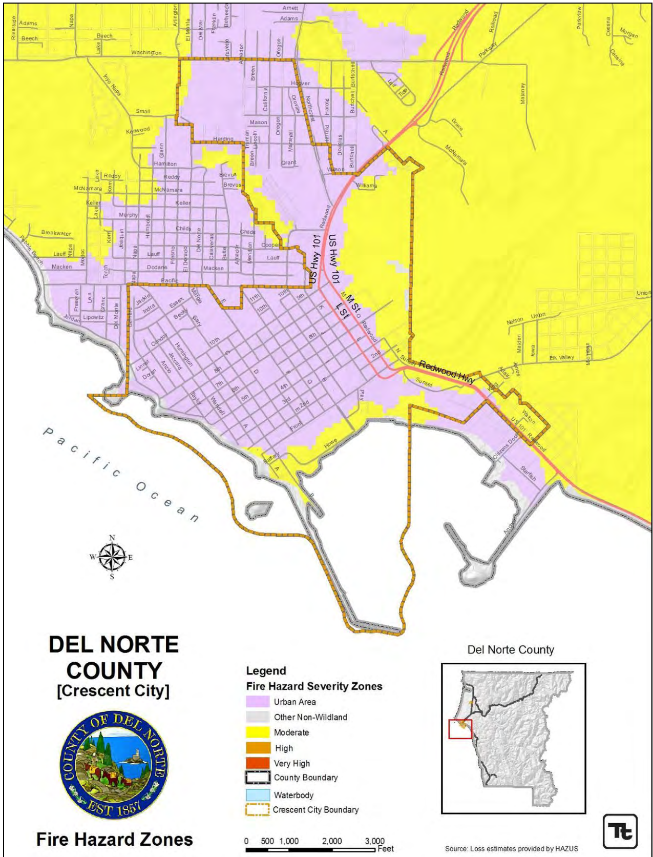
Figure 3-6. Crescent City Fire Hazard Severity Zones
