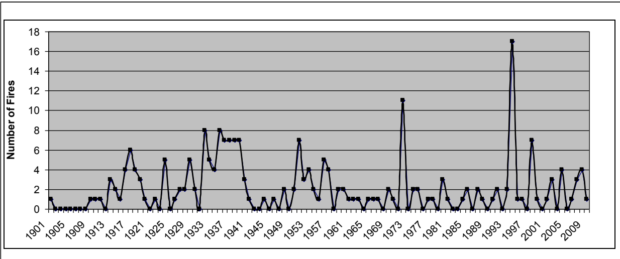
Figure 17-5. Annual Frequency of Fires in Del Norte County, 1901 – 2009
