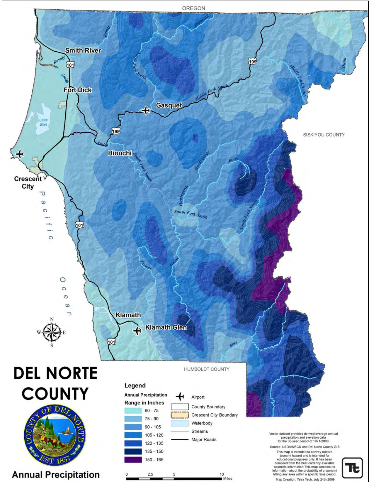
Figure 15-2. Annual Precipitation for Del Norte County
