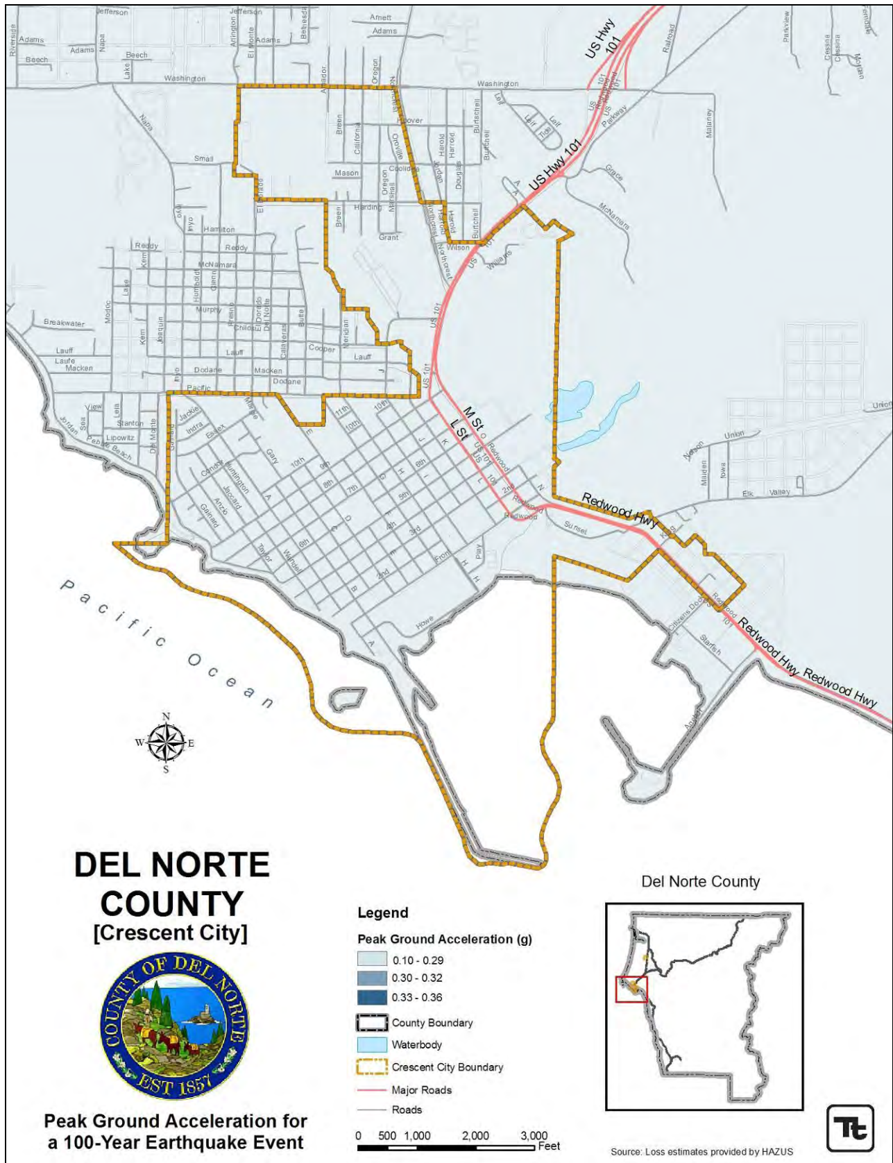
Figure 3-1. Crescent City Earthquake Hazard Areas-100-year probabilistic
