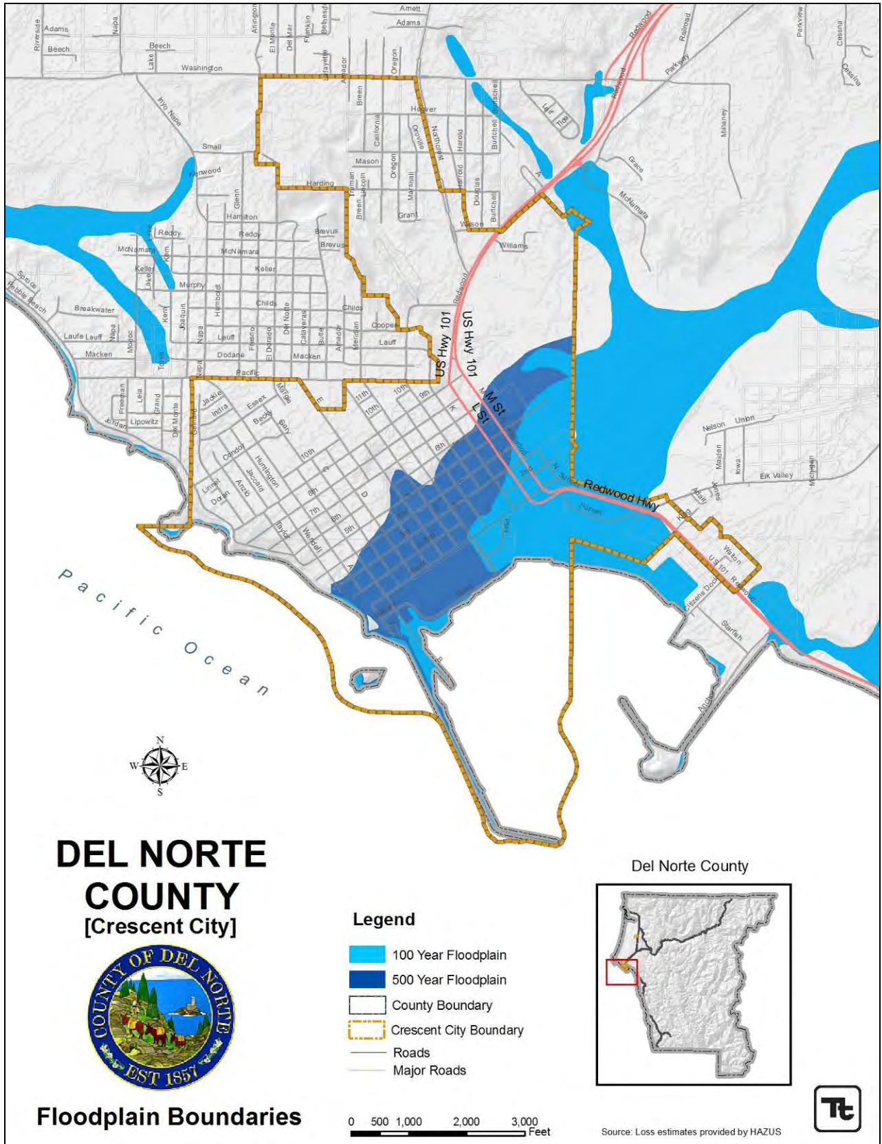
Figure 3-4. Crescent City Flood Hazard Areas
