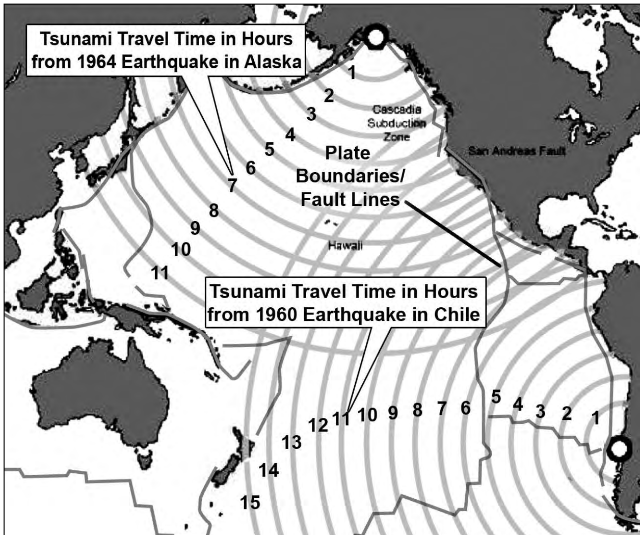
Figure 16-1. Potential Tsunami Travel Times in the Pacific Ocean
