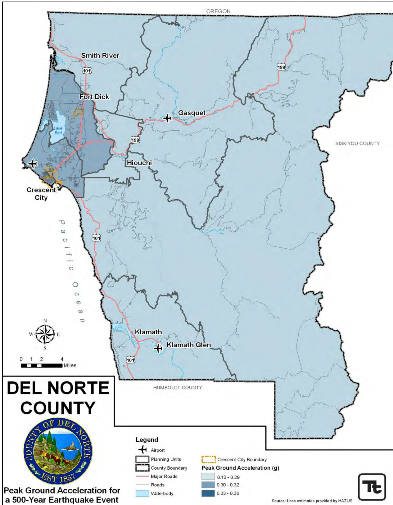
Figure 12-2. 500-Year Probabilistic Ground Motion Map for Del Norte County
