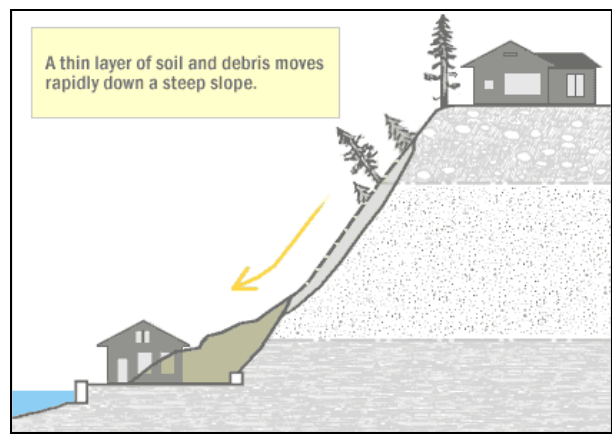
Figure 14-4. Flows
