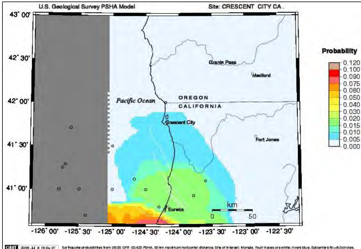
Figure 12-5. Probability of Earthquake with M > 7 Within 5 Years and 50 Kilometers
