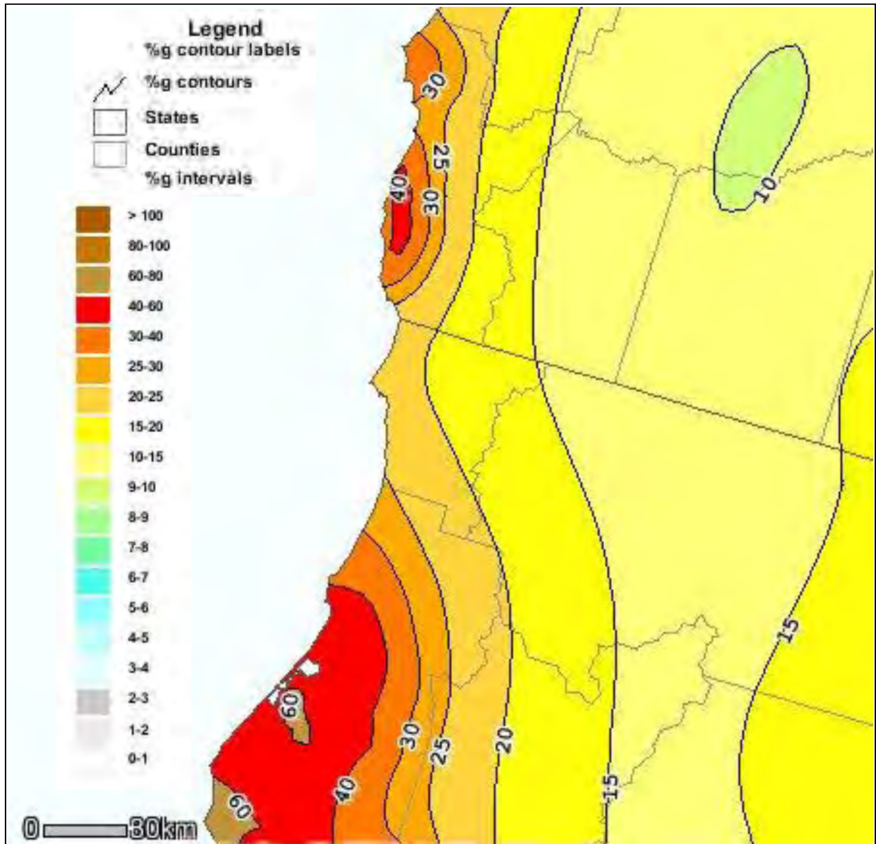
Figure 12-4. Peak Horizontal Acceleration with 10% Probability of Exceedance in 50 Years
