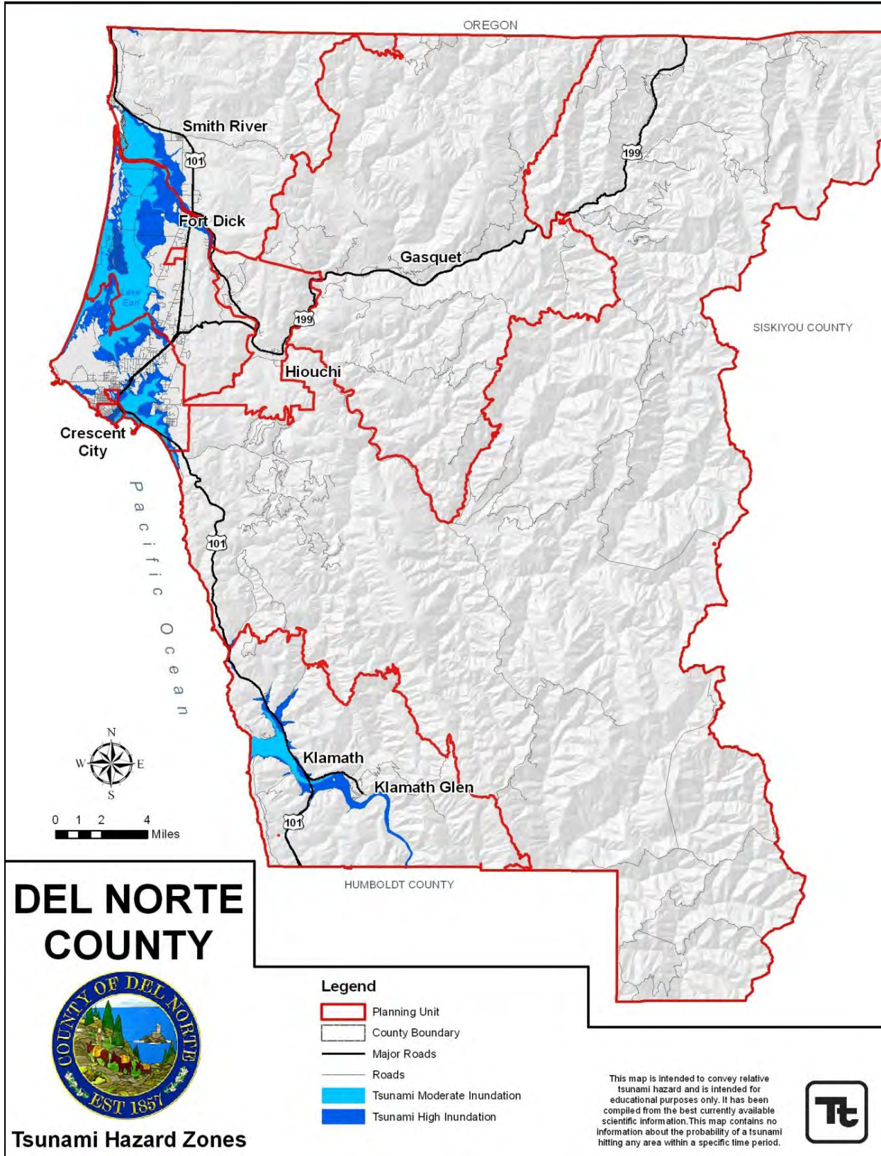
Figure 16-2. Moderate (100 Year) and Highest (500 Year) Tsunami Hazard Zones
