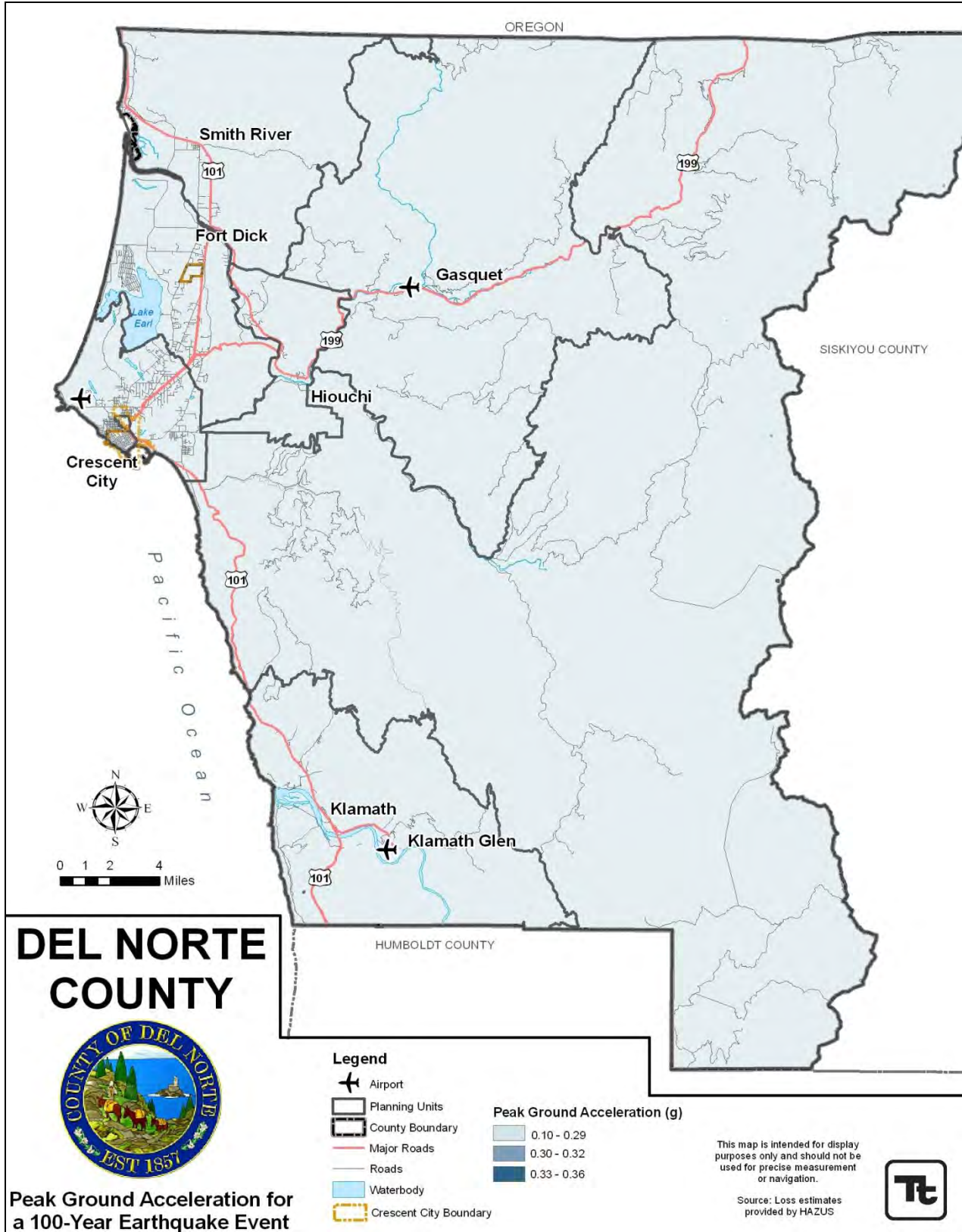
Figure 12-1. 100-Year Probabilistic Ground Motion Map for Del Norte County
