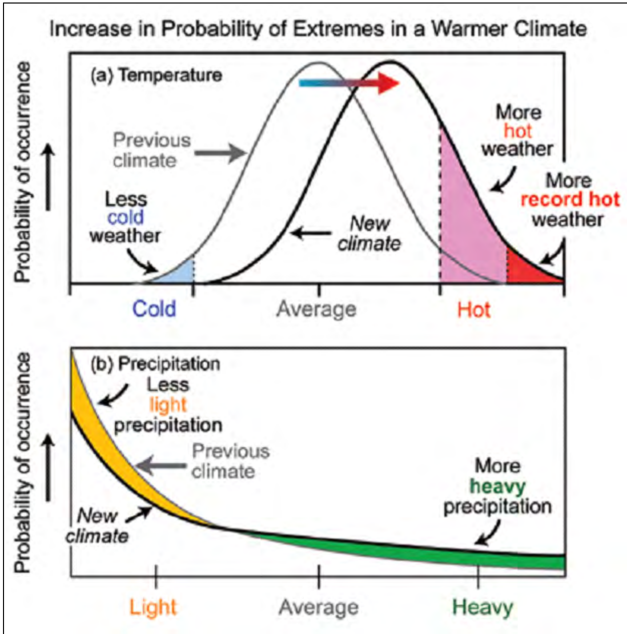
Figure 15-3. Severe Weather Probabilities in Warmer Climates
