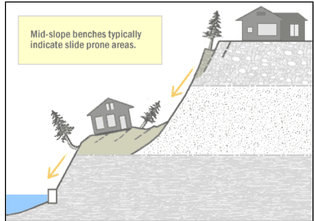
Figure 14-2. Slumps (Small Rotational) Slides
