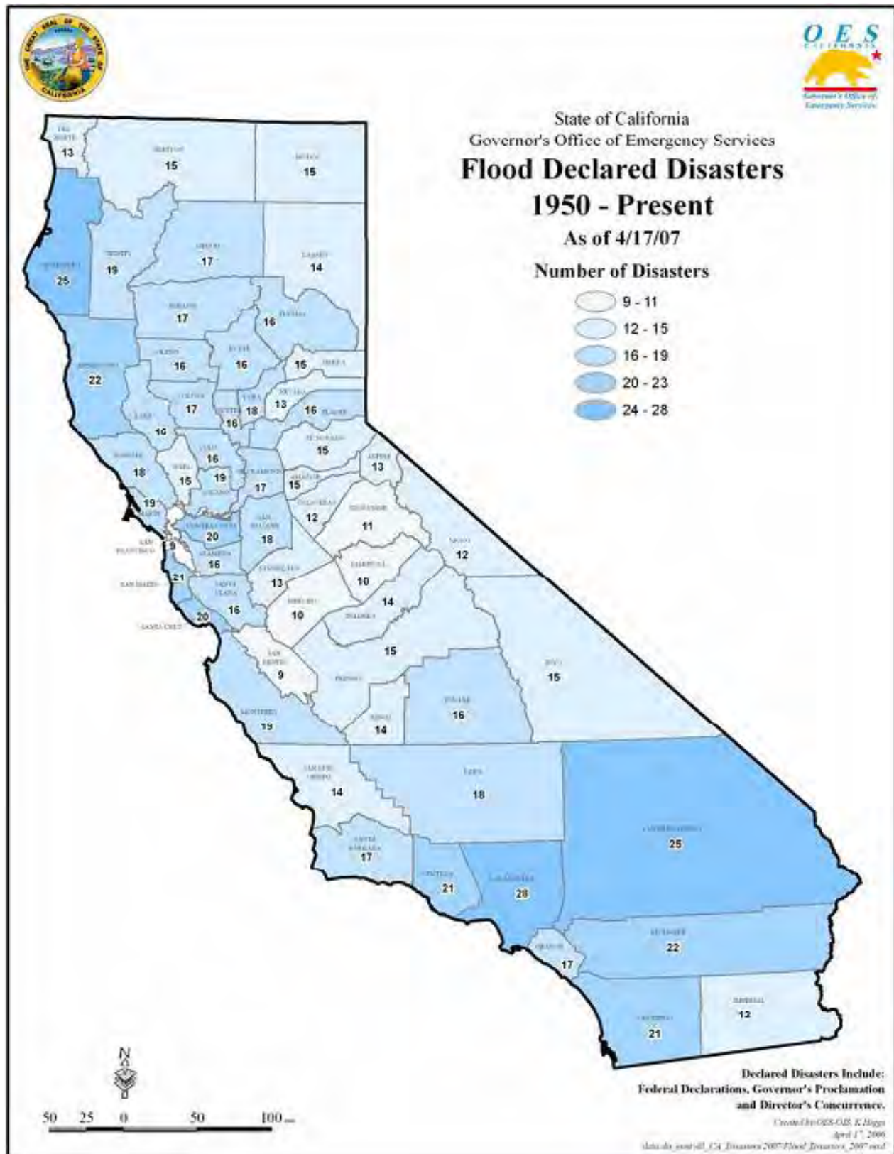
Figure 13-1. Declared Flood Disasters in California, 1950 – 2007
